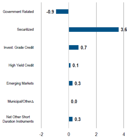
Sector Allocation (Duration in Years)
